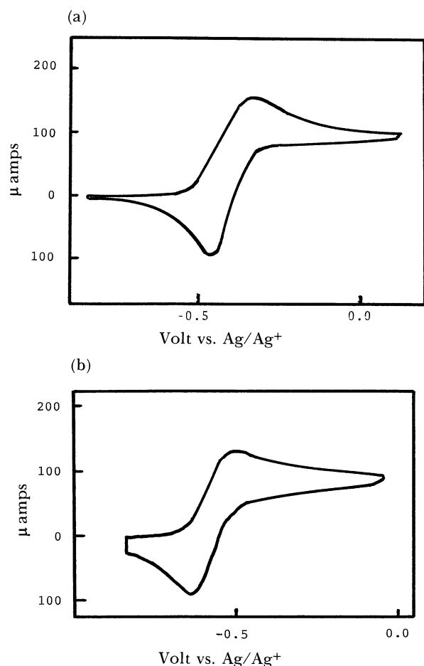
Fig. 1. Cyclic voltammogram of a) [\text{Co}(\text{tip}(\text{b}))]^{2+} and b) [\text{Co}(\text{tip}(\text{b})(\text{py}))]^{2+} . Scan rate 50 \text{ mV}^{-1} . E versus \text{Ag}/\text{Ag}^+ . Counter anion: \text{ClO}_4^- in \text{MeCN} .
